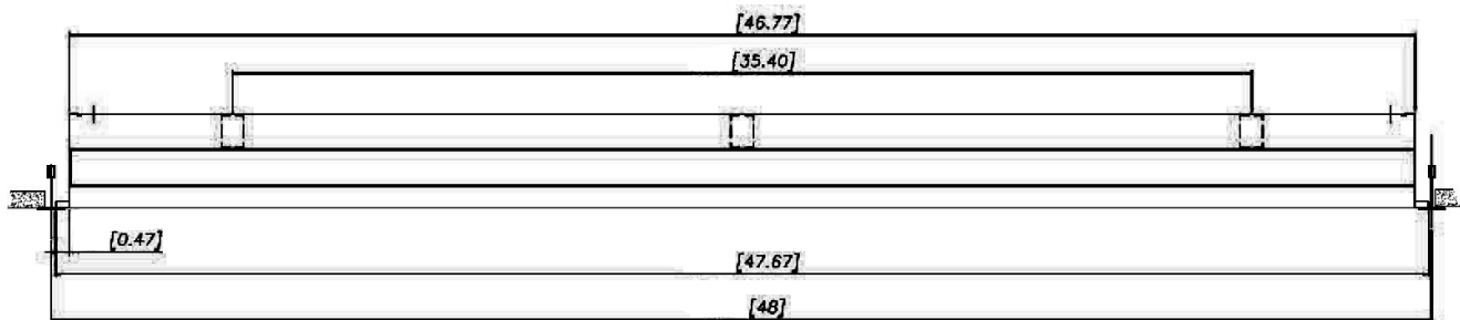
Side View
