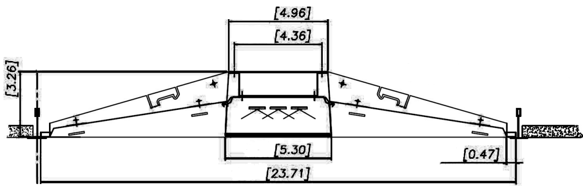
End View
